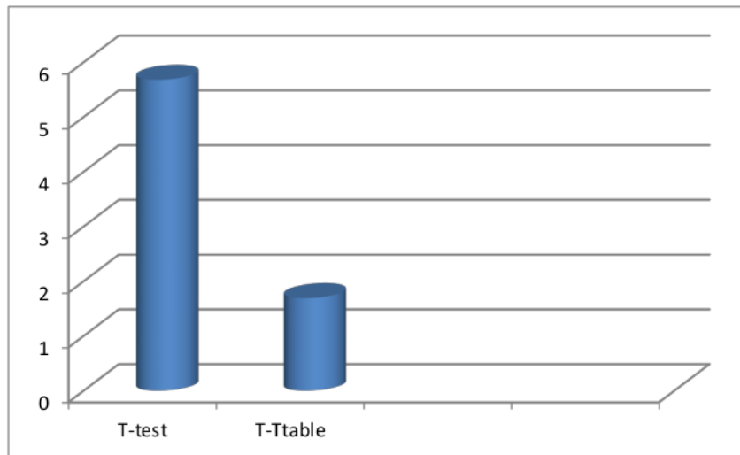
Chart2. The Difference of T-test and T-table
