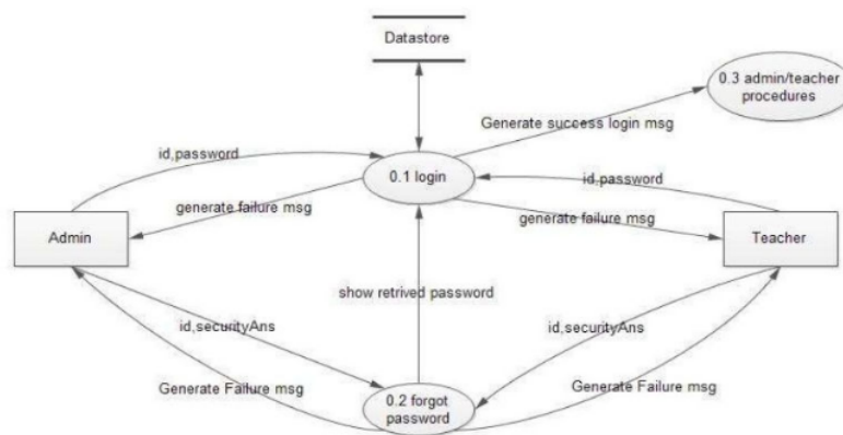
Figure 3. Authentication Module flow diagram
