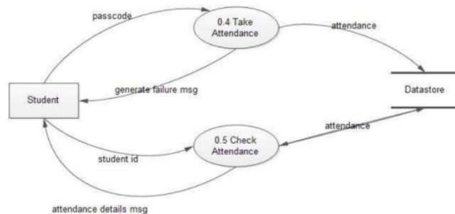
Figure 4. Student attendance module flow diagram
